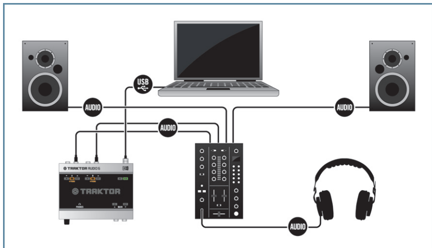
7.4 TRAKTOR AUDIO 6 in a digital DJing setup with a DJing software and an external mixer.
