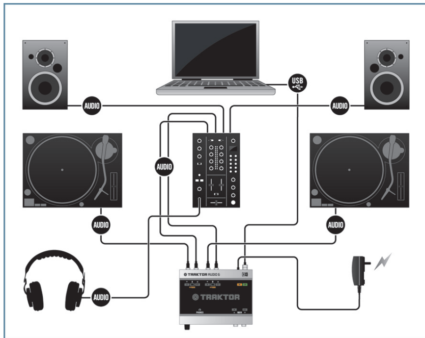
7.5 TRAKTOR AUDIO 6 in a digital DJing setup with a DJing software, turntables with timecode vinyl, and an external mixer.
