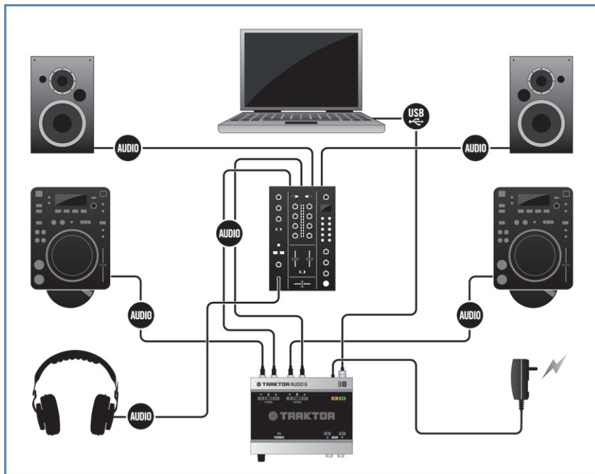
7.6 TRAKTOR AUDIO 6 in a digital DJing setup with a DJing software, CD decks with timecode CDs, and an external mixer.
