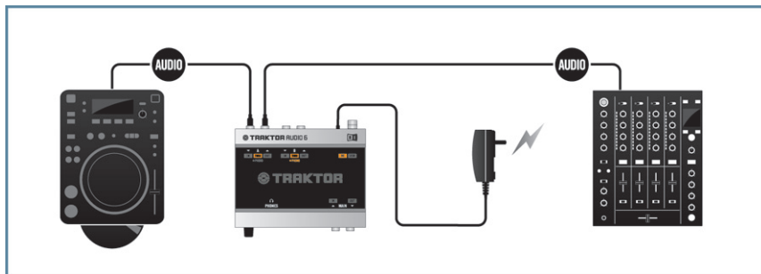
7.2 TRAKTOR AUDIO 6 in an analog DJing setup with a CD deck and a mixer.
